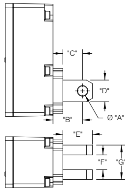
Rear Clevis (KSRC-60, KSMC-60)
