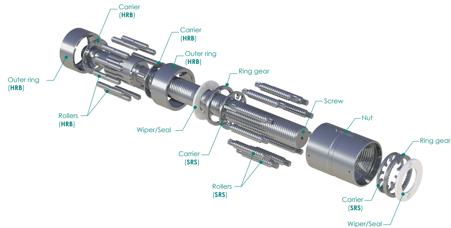
Fig. 6.2: a split Roller Screw with integrated HRB on the shaft (HRA - s)
