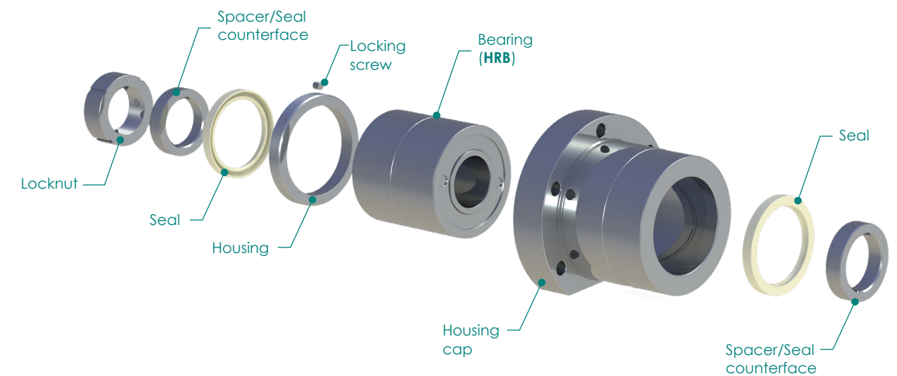
Fig. 8.4: a split Support Bearing Unit with a HRB ( HHF )
