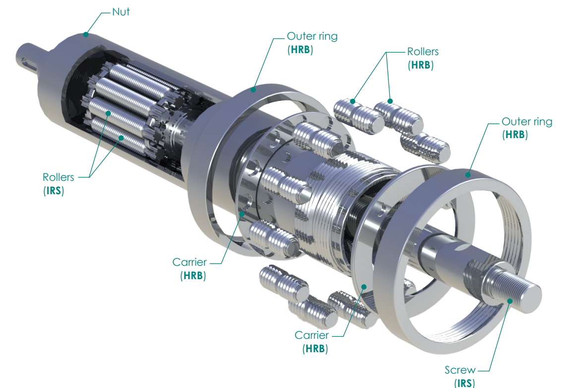
Fig. 6.4: a split Roller Screw with integrated HRB on the nut ( HRA - i )
